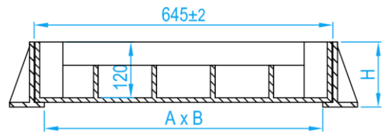
SECTION VIEW
