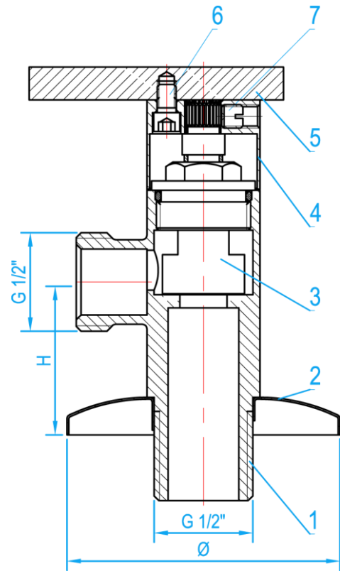
SECTION VIEW
