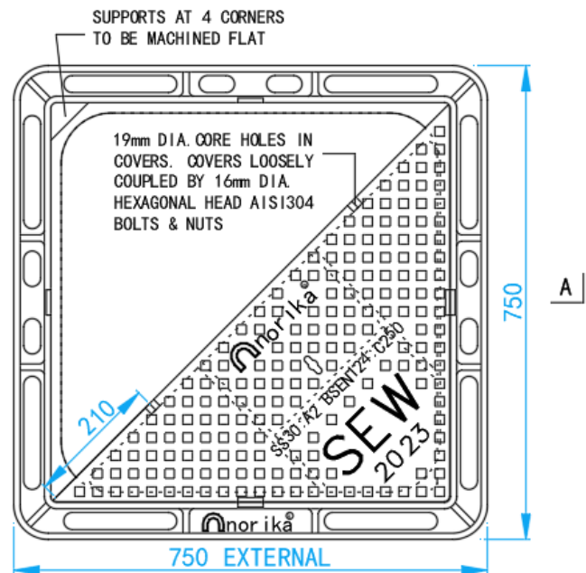
HALF COVER REMOVED TOP VIEW
