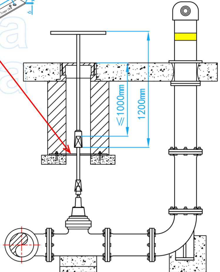
INSTALLATION ASSEMBLY
