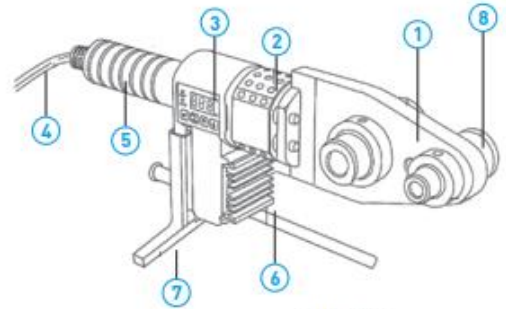
3-D VIEW
