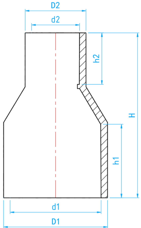
CROSS SECTION VIEW
