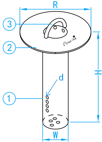
3-D VIEW
